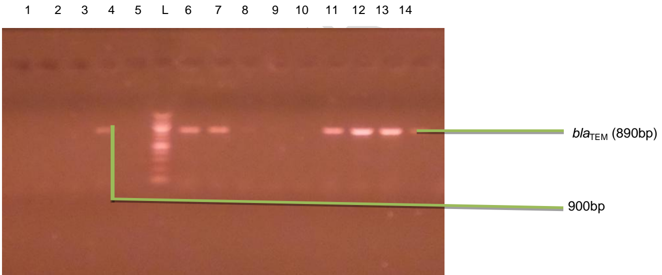
Plate 3: Agarose gel electrophoresis showing the bla TEM bands, lanes 4, 6, 7, 11, 12, 13 and 14 represent bla TEM gene bands while L represents the 1000bp molecular ladder.
