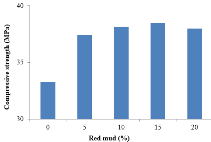
Fig. 2. Compressive strength at different % of red mud [28]
