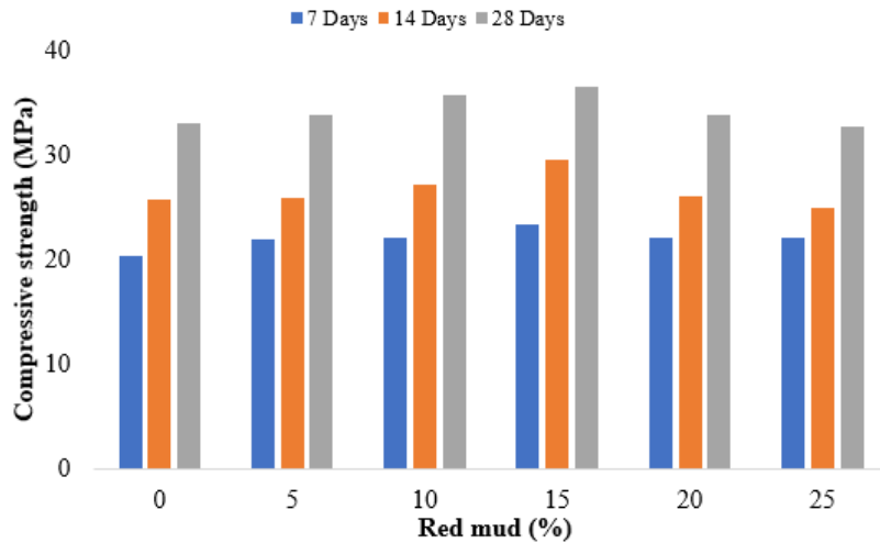
Fig. 1. Compressive strength at various age of curing [19]
