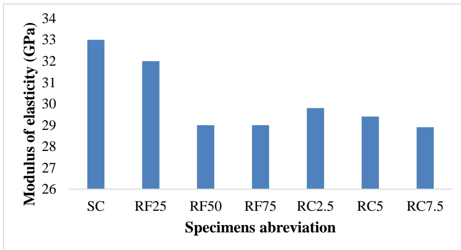
Fig. 9. Modulus of elasticity of different mixes [29]
