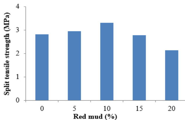
Fig. 5. Split tensile strength results [18]
