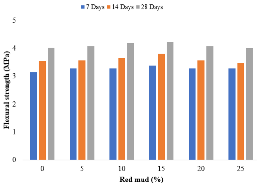
Fig. 6. Flexural strength at different ages [19]
