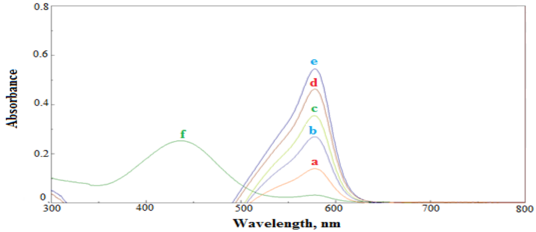
Fig. 6. Final spectrum of (700, 500, 300, 200 and 100) \mu\text{g} FSD for the 2nd method measured against Blank (a, b, c, d and e), and Blank measured against distilled water (f).
