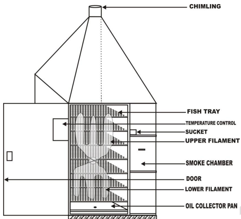
Figure 3: Schematic Diagram of Electric Fish Smoking Kiln
