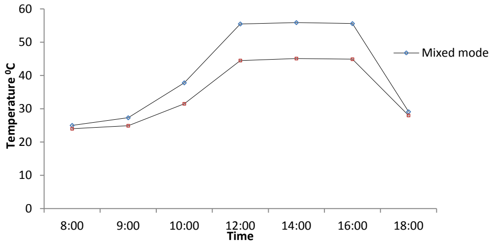
Figure 5. Variation of drying chamber temperature with local time for unloaded dryers
