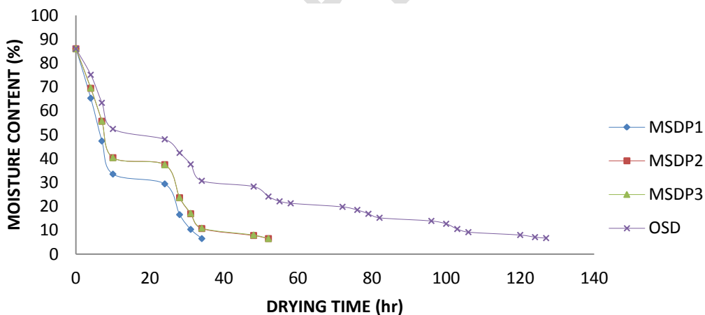
Figure 8 Drying characteristics of Okra slices in mixed mode solar dryer for and Open Sun Drying
