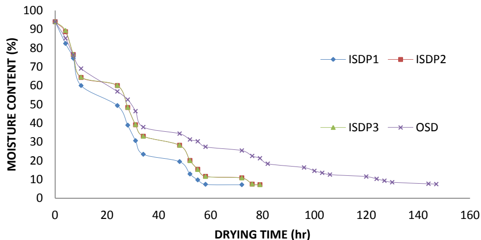
Figure 7. Drying characteristics of Tomato Slices in Indirect mode solar dryer for vegetables and Open Sun Drying
