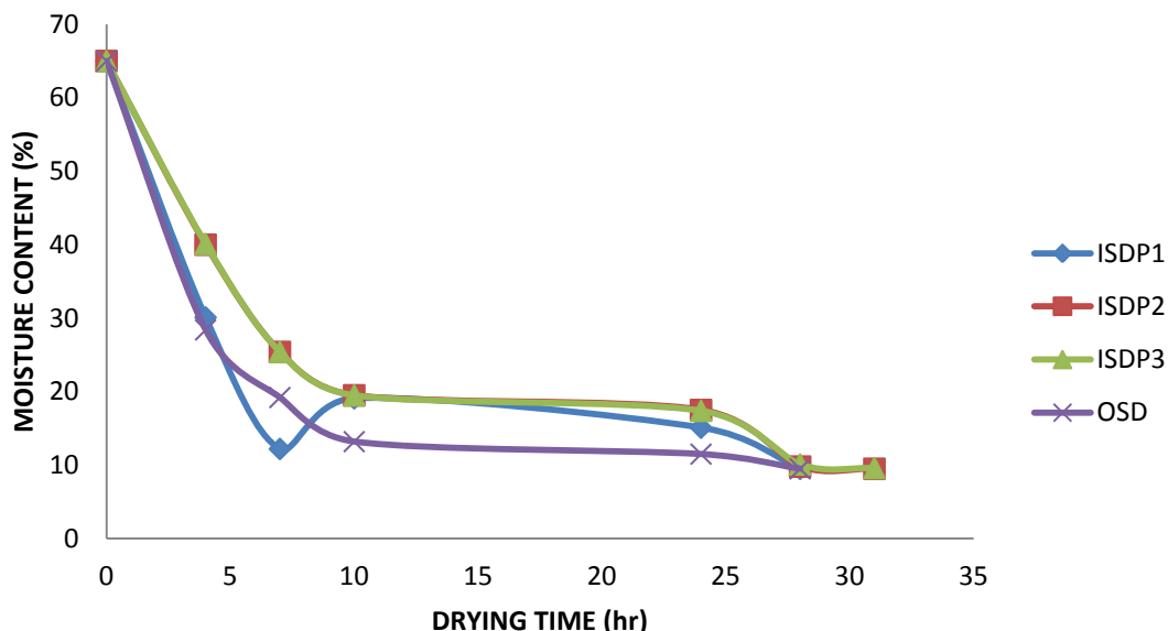
Figure 11. Drying characteristics of baobab leaves in indirect mode solar dryer and open sun drying
