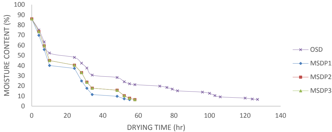
Figure 9 Drying characteristics of Okra slices in Indirect mode solar dryer for vegetables and Open Sun Drying
