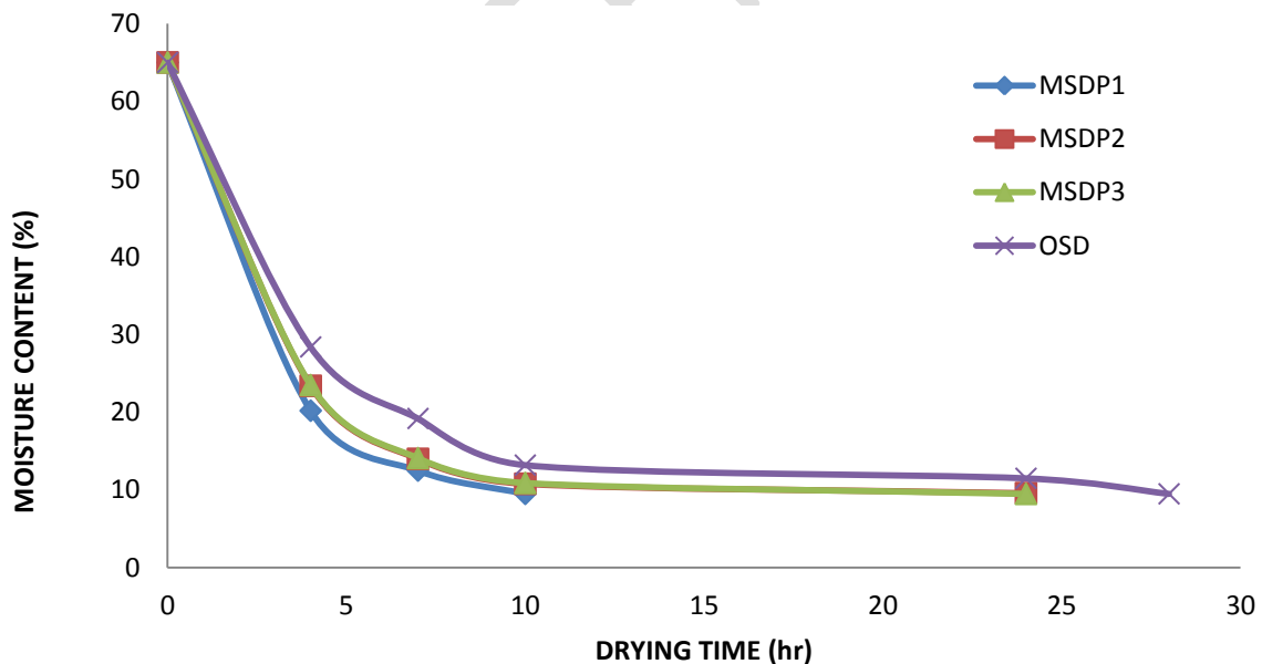
Figure 10 Drying characteristics of baobab leaves in mix-mode solar dryer and open sun drying
