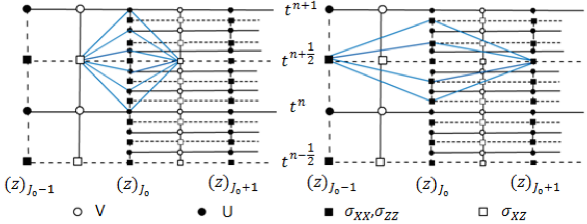
Figure 6: 2D (t, z) projection of embedded stencils used to update the solution from the instant t^{n+1/2} to t^{n+1} . Stress component at the interface is updated with the stencil.
