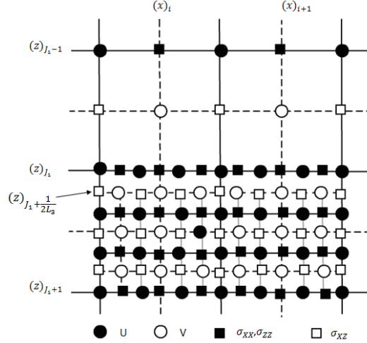
Figure 7: The grid of the spatial mesh refinement interface (x_3)_{J_1} .
