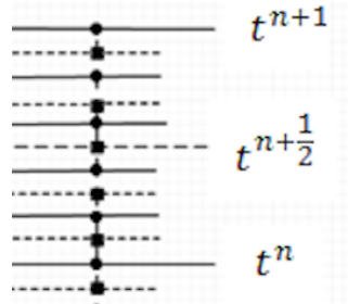
Figure 4: A section of the time grid
