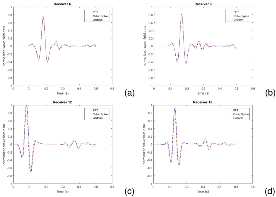
Figure 11: Comparison between wave fields generated by fast Fourier interpolation and cubic smoothing spline interpolation.
