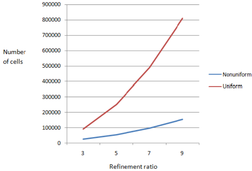
Figure 10: Number of cells as a function of refinement ratio.
