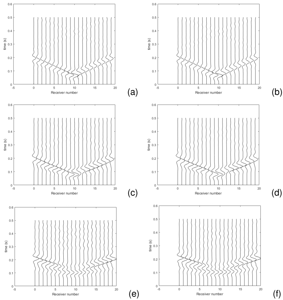
Figure 9: Wave fields from the mesh refinement method (non uniform mesh) at (a) 0.5 m depth, (c) 6.5 m depth, and (e) 16.5 m depth. Wave propagation from the uniform mesh at (b) 0.5 m depth, (d) 6.5 m depth, and (f) 16.5 m depth.
