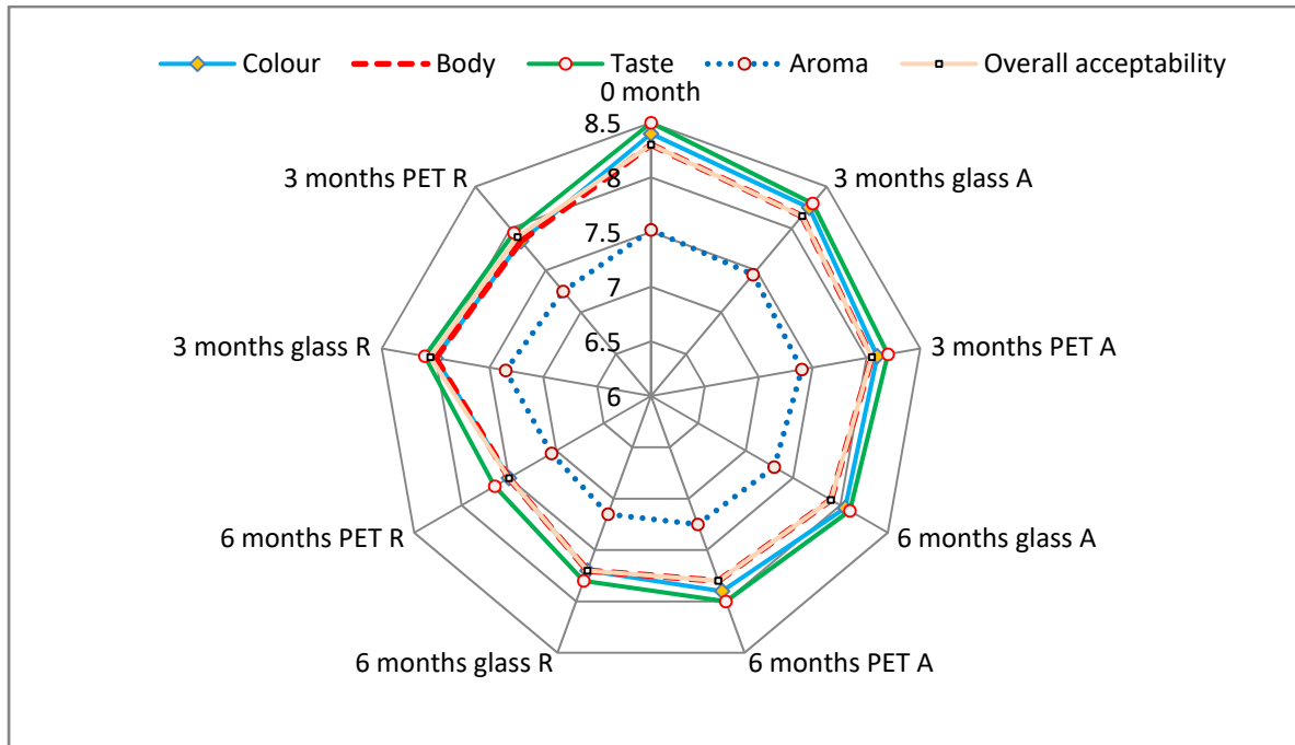
Figure 3. Effect of storage and packaging on sensory characteristics of rhododendron appetizer stored under ambient (A) and refrigerated (R) conditions
