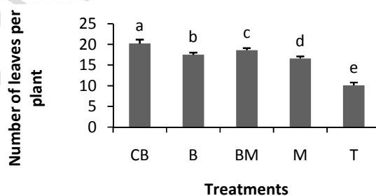
Figure 5 : Leaf production at 7 months after sowing CB : compost, B : bagasse, BM : bagasse-molasses mixture, M : molasses ; T : unfertilized plants. Values of bands affected by different letter are significantly different ( p < 0.0001 ).
