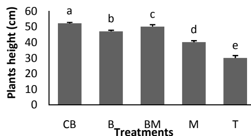
Figure 4 : Moabi plants height at 7 months after sowing CB : compost, B : bagasse, BM : bagasse-molasses mixture, M : molasses ; T : unfertilized plants. Values of bands affected by different letter are significantly different p < 0.0001 .
