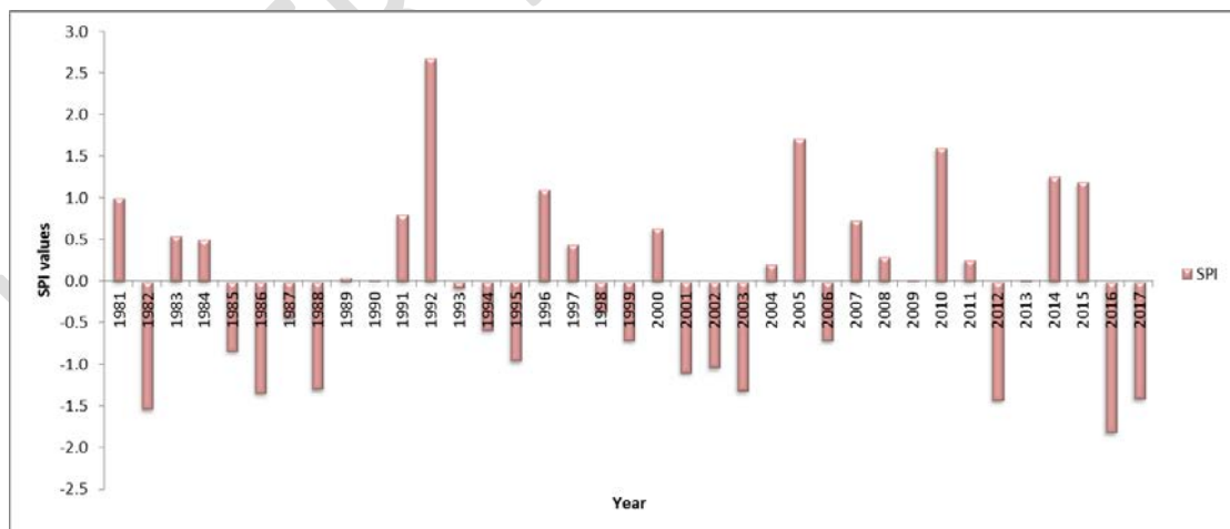
Fig. 5. 12-month time scale basis drought results using SPI method in PAP hilly areas
