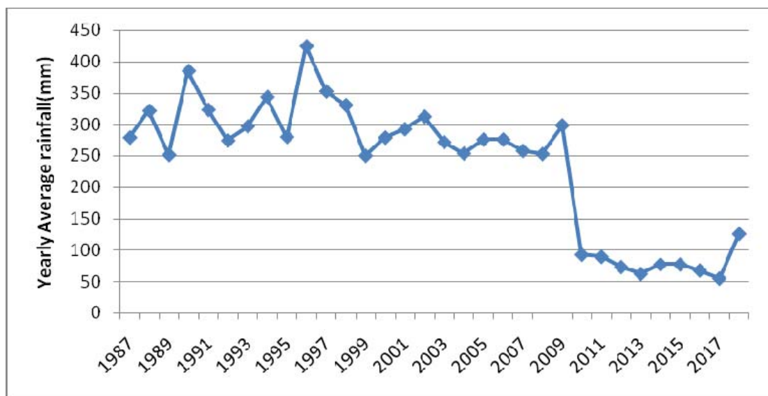
Fig 4 Average annual rainfall trends for Mbita: 1987-2017
