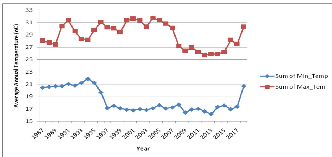
Fig 6: Yearly trend of temperature data for Mbita: 1987-2017
