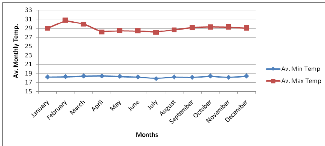
Fig 5 Average monthly temperature trends data for Mbita: 1987-2017
