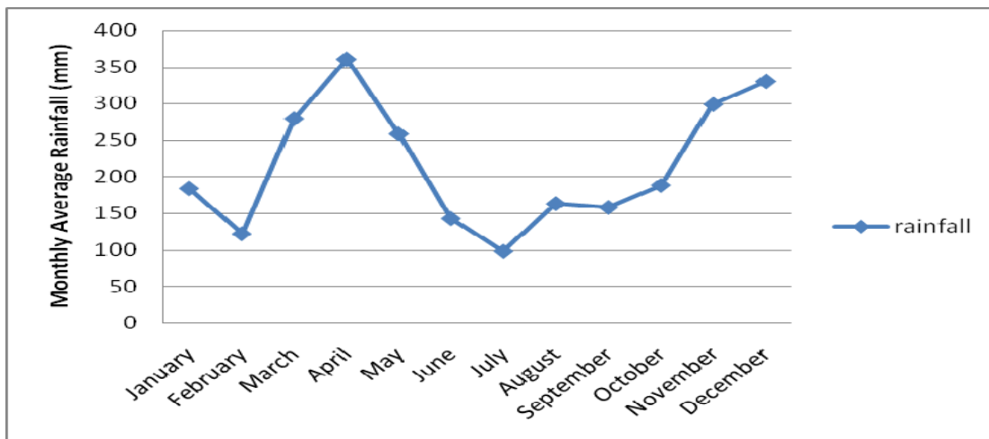
Fig 3. Average monthly trends of rainfall data for Mbita (From 1987 to 2017).
