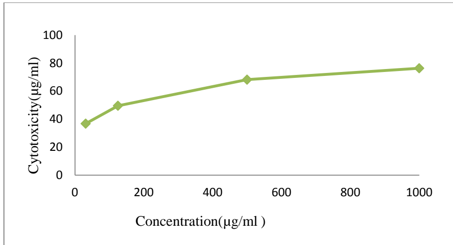
Figure 2: ABTS radical scavenging activity of the dry sample extracted from ethyl acetate fraction of Moringa oleifera flowers
