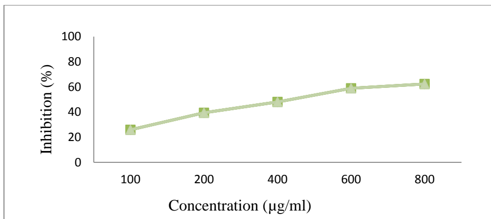
Figure 3: The human red blood cell membrane Stabilization activity of the dry sample extracted from ethyl acetate fraction of Moringa oleifera flowers
