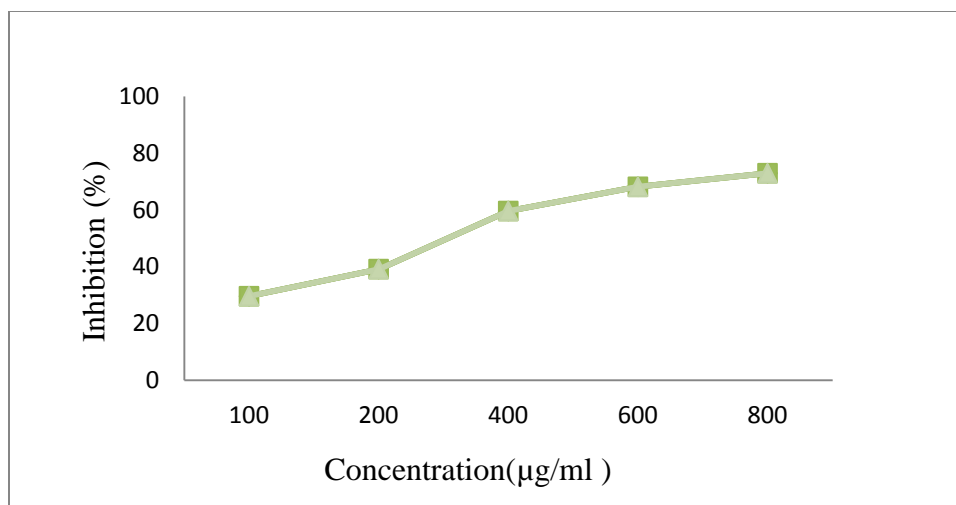
Figure 4: The Inhibition of Albumin Denaturation activity of the dry sample extracted from ethyl acetate fraction of Moringa oleifera flowers
