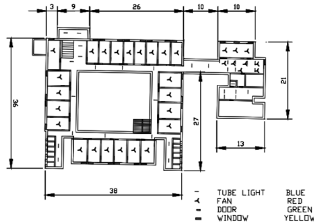
Fig. 1. Layout of an Undergraduate hostel
