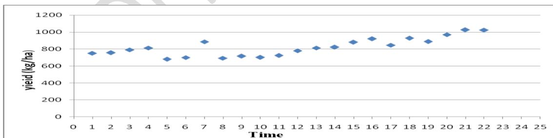
Figure 2: Scatter plot for yield of rabi food grains in Odisha
