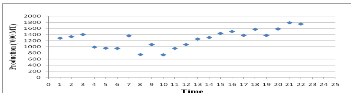
Figure 3: Scatter plot for production of rabi food grains in Odisha
