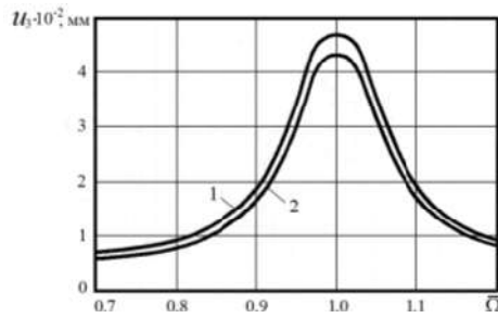
Fig.5 Forced Vibration amplitudes with damping
