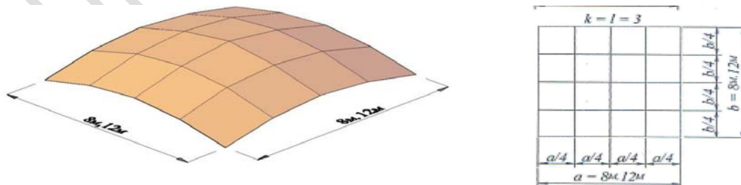
Fig.2. Mathematical model of folded shell
