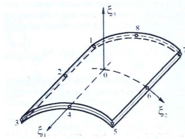
Fig.1. Eight node Iso-parametric curvilinear element
