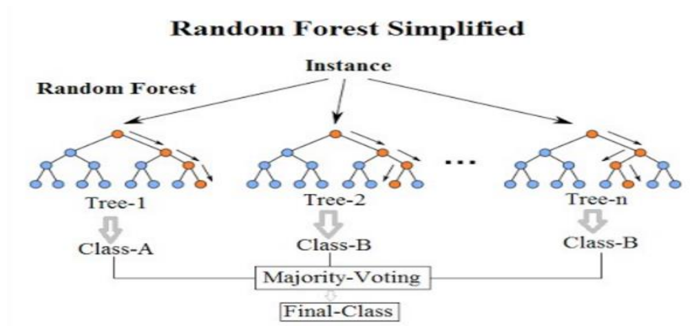
Figure 2 Random Forest
