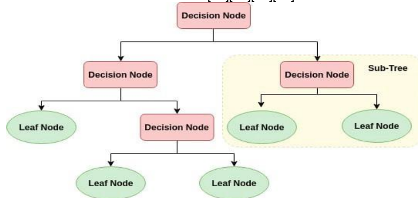
Figure 1 Decision Tree
