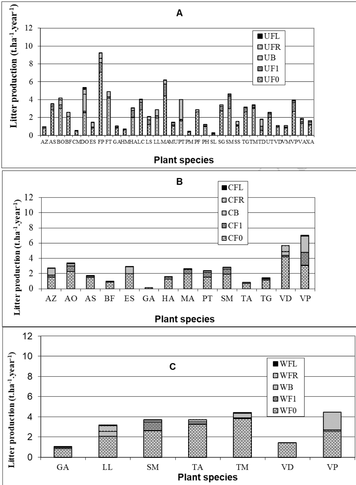
Figure 1: Litter production ( t \cdot ha^{-1} \cdot yr^{-1} ) according to category at Dang (A), Biskewal (B) and Wakwa (C). Leaf litter of year n (F0), previous years (F1), wood litter (B), fruits and seed litter (FR), and Flower litter (FL). Dang (U), Biskewal (C), and Wakwa (W).
