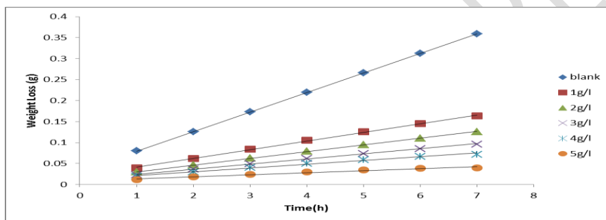
Figure 1. Plot of weight loss against time for pipeline steel corrosion in 0.5 M HCl with varying concentrations of CCC aqueous extract at 303 K.
