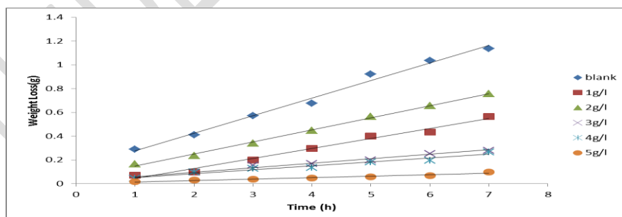
Figure 2. Plot of weight loss against time for pipeline steel corrosion in 0.5 M HCl with varying concentrations of CCC aqueous extract at 333 K.
