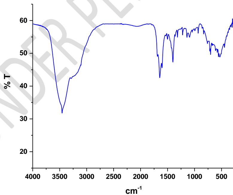
Fig. 4. IR Spectrum of the complex, [\text{CuL}(\text{CH}_3\text{COO})_2(\text{H}_2\text{O})]
