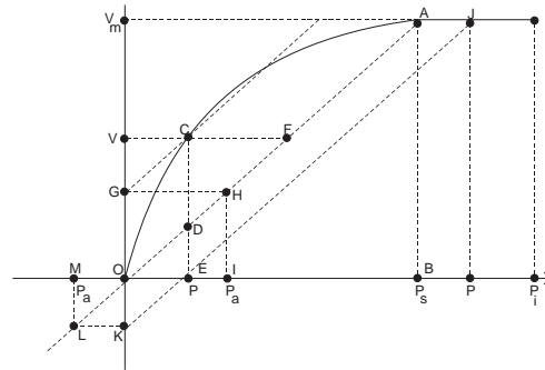
Figure 3: Graphical analysis of the developed adsorption isotherm
