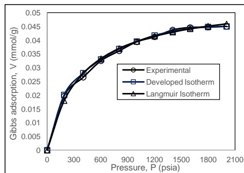
Figure 7: Generalization of the developed isotherm for methane adsorption on Turkey's shale sample at 25 °C
