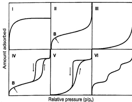
Figure 1: Main types of gas physisorption Isotherms [xx]. (Source: IUPAC, 1985)
