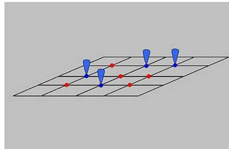
Figure 2: Physical Depiction (Schematic) of Adsorption in the New Model [xx]. (Source: Langmuir, 1916)
