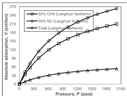
Figure 15: Plot of adsorption versus pressure for methane and nitrogen competitive adsorption on Tiffany mixed coal sample at 130 °F as predicted by Langmuir isotherm
