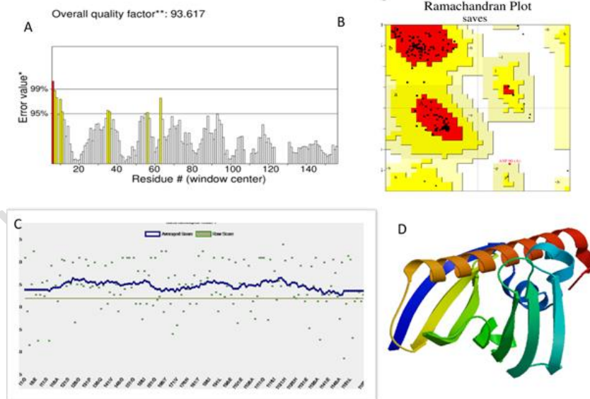
Figure 3: VERIFY 3D analysis indicates that 100% of the residues have average 3D-ID score \geq 0.2 . D) 3-D structure of Hazel allergen (Cor a1) modelled through SWISS-MODEL.
