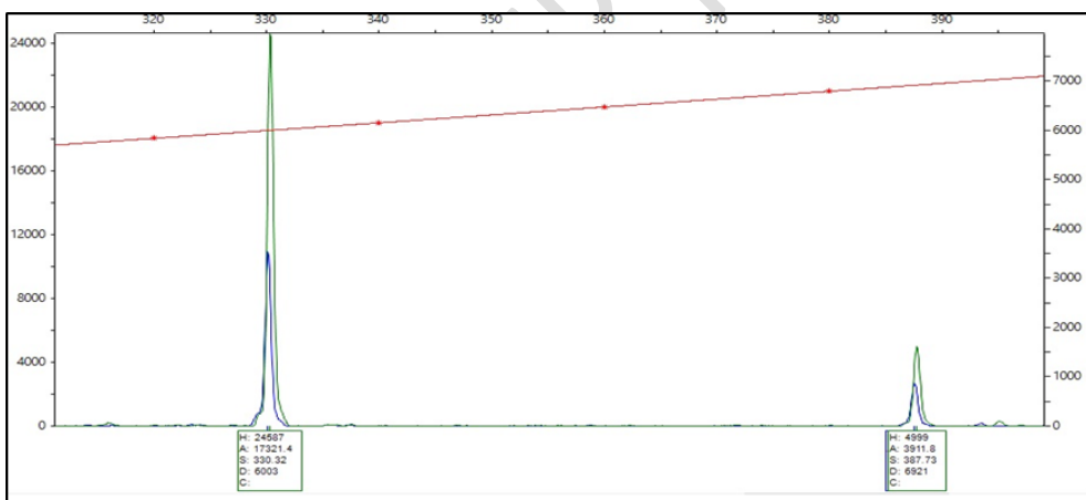
Figure-2: Fragment analysis result of heterozygous FLT - ITD positive patient having 330 and 387 bp bands (Blue: FAM, Green: HEX)
