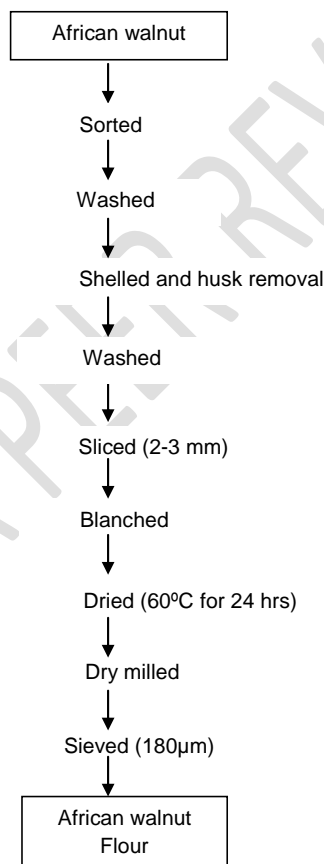
Fig 1: Flow chart for the production of walnut flour Source: [11]
