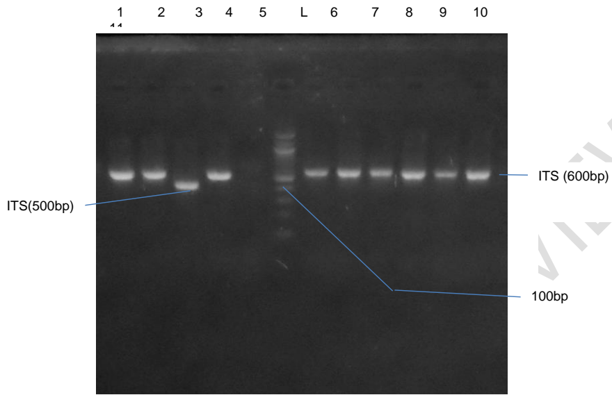
Figure 1.: Agarose gel electrophoresis showing the amplified ITS fragment of the fungal isolates. Lanes 1-4, 6-11 represent the ITS bands at 400bp and 600bp while lane L represents the 100bp molecular ladder.
