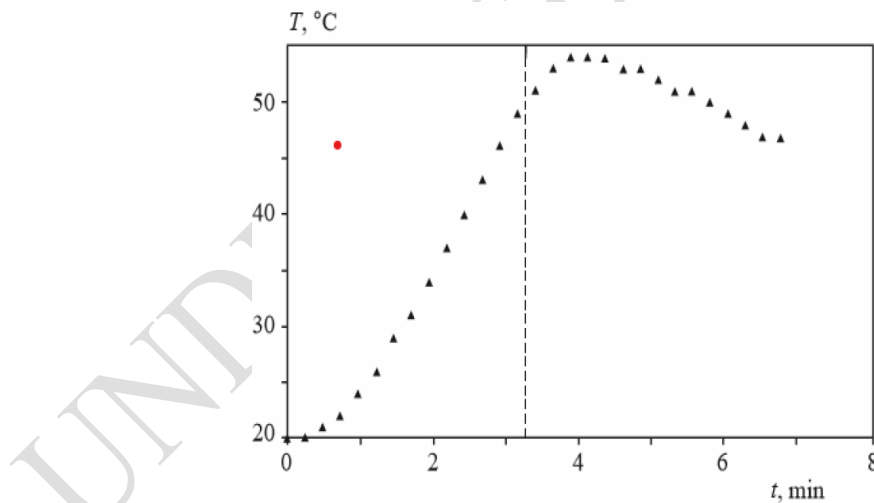
Figure 2. Time dependence of the temperature of a part of the surface of an ultrasonically heated brass rod (open holder). Ultrasound frequency 131.28 kHz. The dashed line indicates the moment when the ultrasound was switched off.
