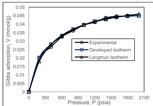
Figure 7: Generalisation of the developed isotherm for methane adsorption on Turkey's shale sample at 25 °C
