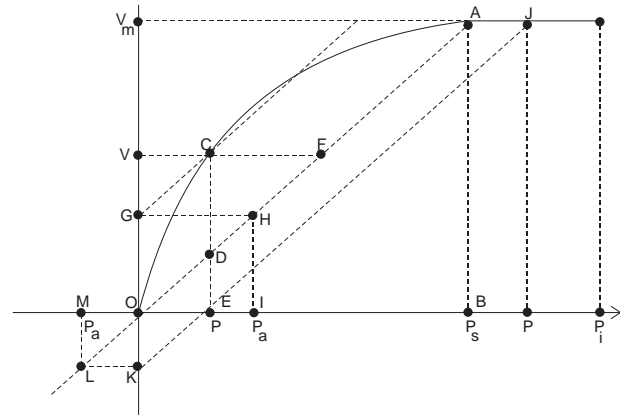
Figure 3: Graphical analysis of the developed adsorption isotherm
