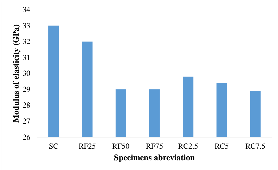
Fig. 9 Modulus of elasticity of different mixes [29]
