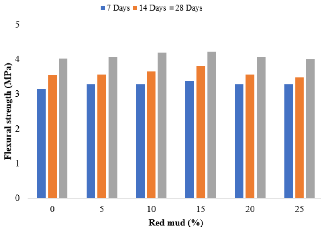
Fig. 6 Flexural strength at different ages [19]
