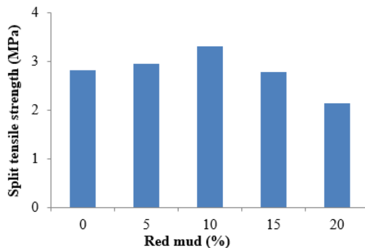
Fig. 5 Split tensile strength results [18]
