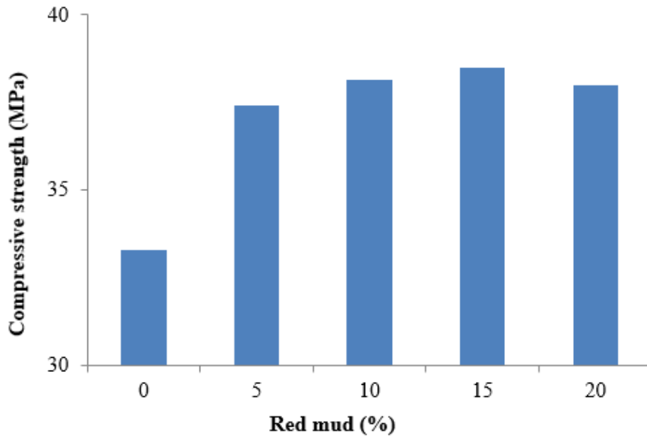
Fig. 2 Compressive strength at different % of red mud [28]
