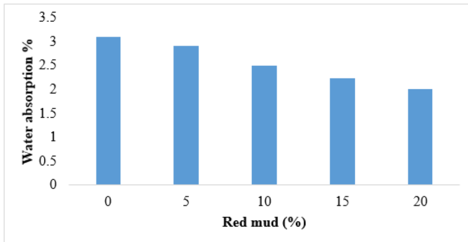
Fig. 8 Water absorption at different % of red mud containing concrete [66]
