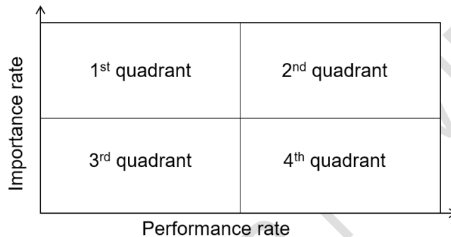
Fig. 1. Four quadrants of Cartesian diagram
