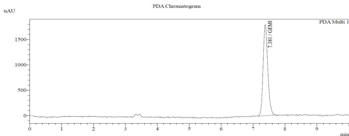
Figure 5c. Chromatogram of Gemigliptin API solution
