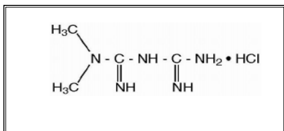
Figure. 1 Metformin Hydrochloride
