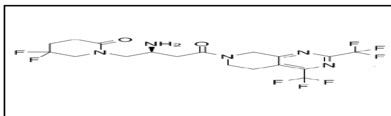
Figure-2 Gemigliptin
