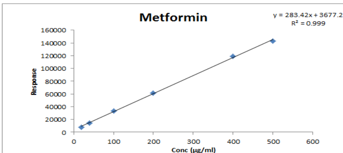
Figure 6. Standard calibration curve of Metformin Hydrochloride
