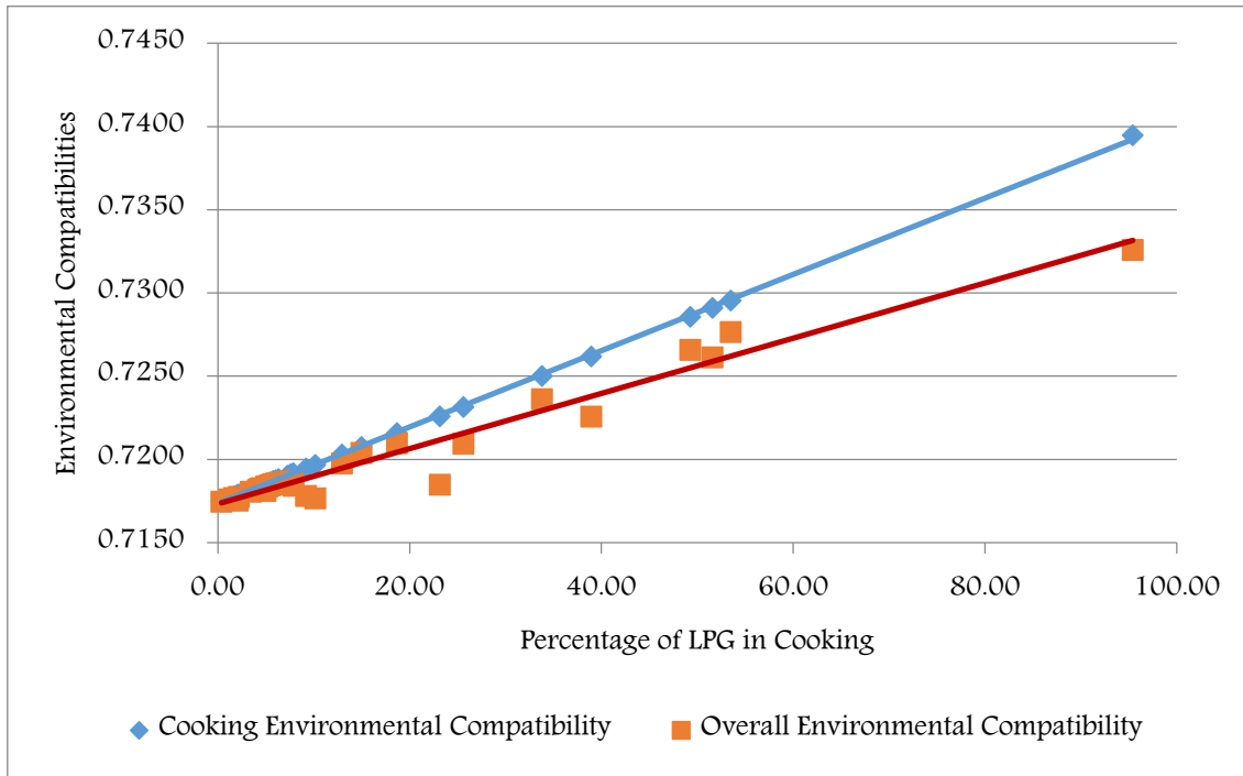
Fig. 5. Effects of LPG Percentage in Cooking on Environmental Compatibilities
