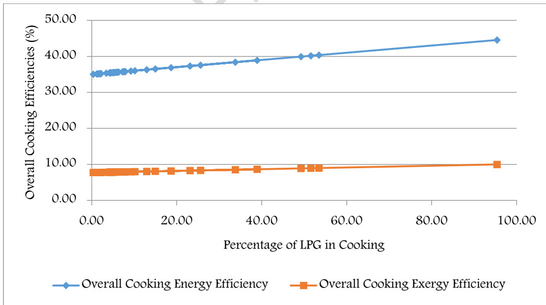
Fig. 6. Effects of LPG Percentage in Cooking on Overall Cooking Efficiencies
