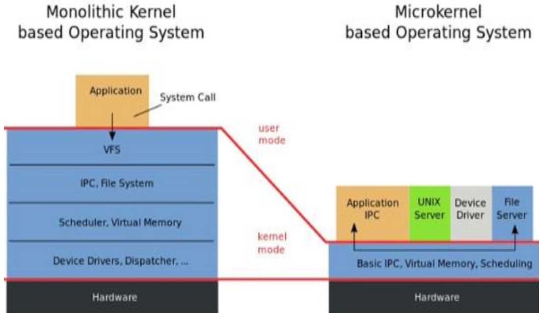
Fig. 2. The architecture of a Transform of Monolithic Kernel to Microkernel [41].
