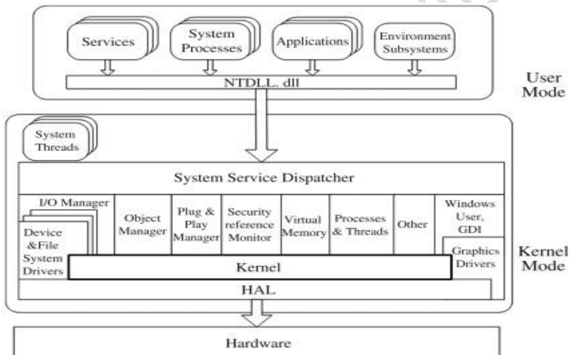
Fig. 1. The abstract view of a kernel [5].
