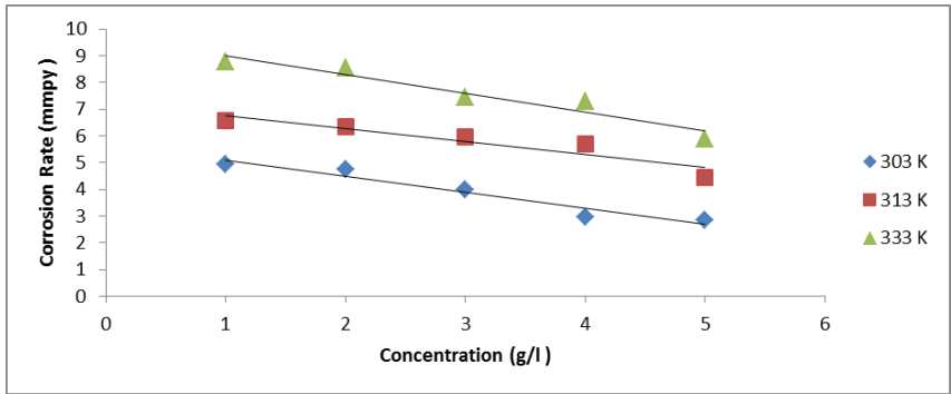
Figure 3: Plot of Corrosion Rate against Concentration of CCC extract on the corrosion of pipeline steel in 0.5 M HCl at different temperatures
