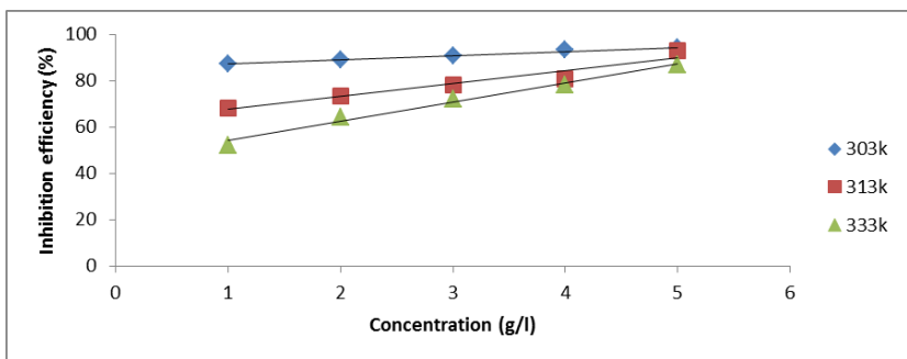
Figure 4. Plot of corrosion inhibition efficiency against concentration of CCC extract on the corrosion of pipeline steel in 0.5 M HCl at different temperature.
