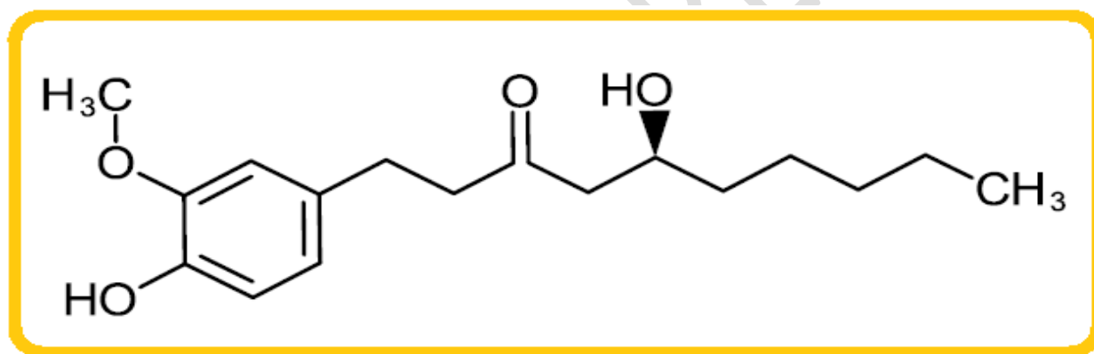
Figure 1. The chemical structure of 6-gingerol ( http://www.chemspider.com/Chemical-Structure.391126.html )
