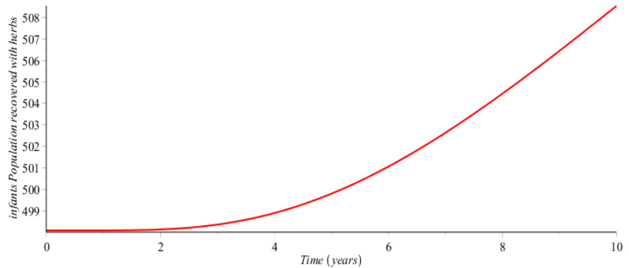
Figure. 2: Simulation of Recovered Infants Population from infectious diseases using Medicinal plants (Herbs)
