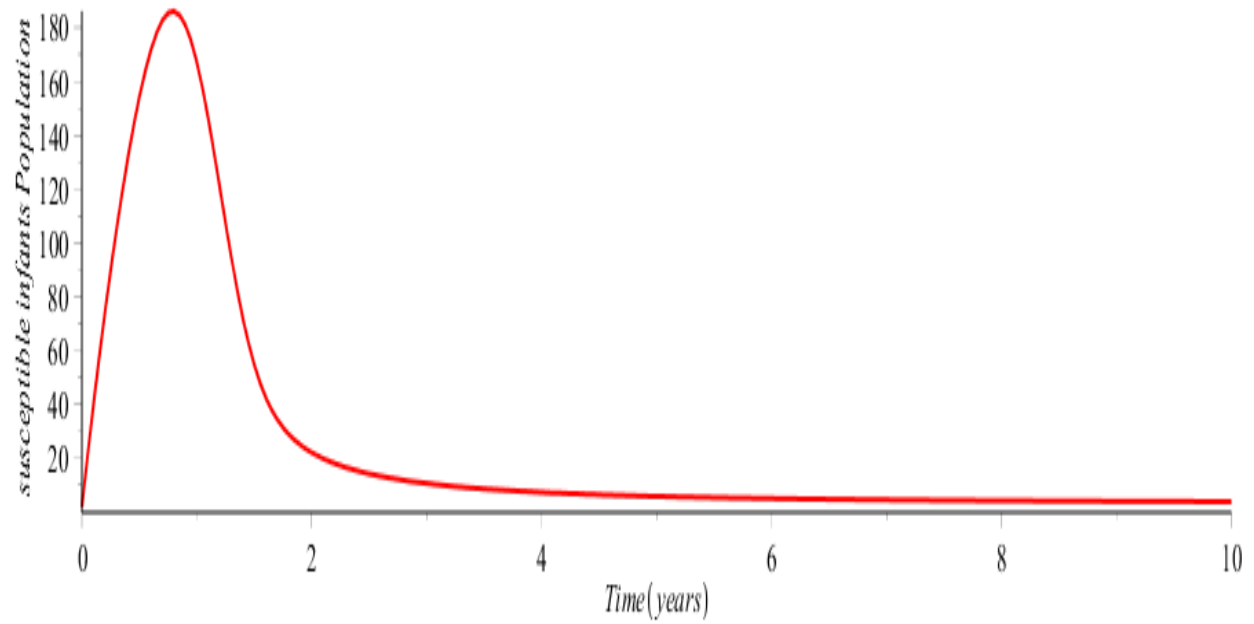
Figure 1: Simulation of susceptible infant's population
