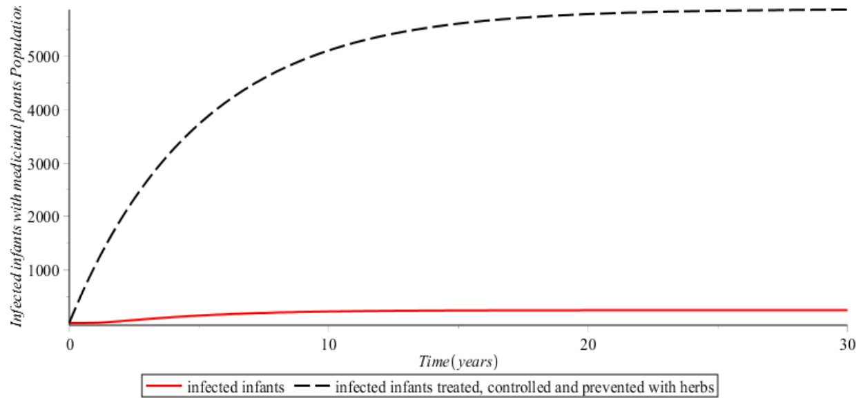
Figure 3: Simulation of infected infants treated, controlled and prevented with medicinal plants
