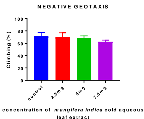
Fig 3: the climbing performance of M. indica cold aqueous leaf extract-treated flies.
