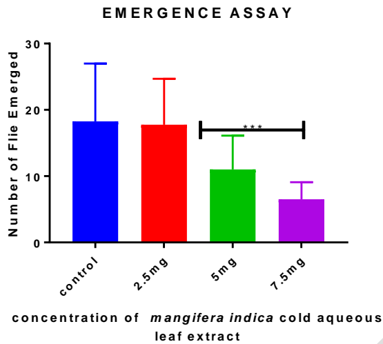
Fig 4: The number of emerged adult flies from the eggs of M. indica cold aqueous leaf extract-treated flies.
