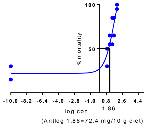
Fig 1: LC 50 of M. indica cold aqueous leaf extract in Flies
