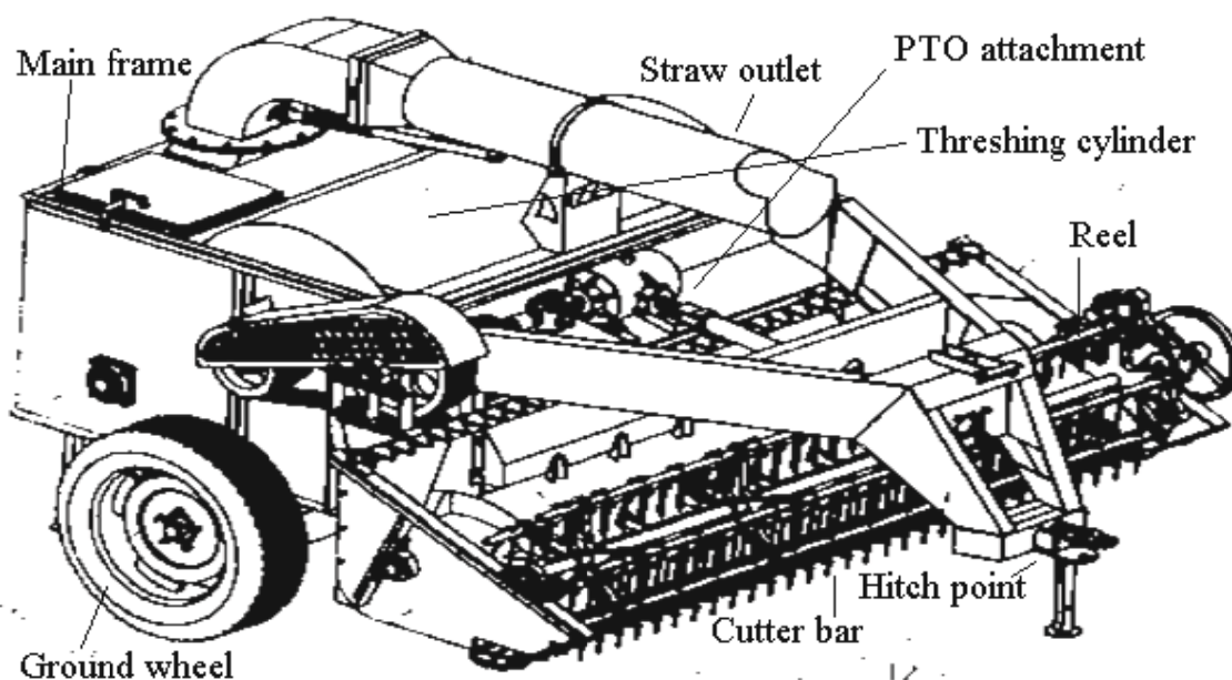
Figure 1: Schematic view of a Straw reaper combine
