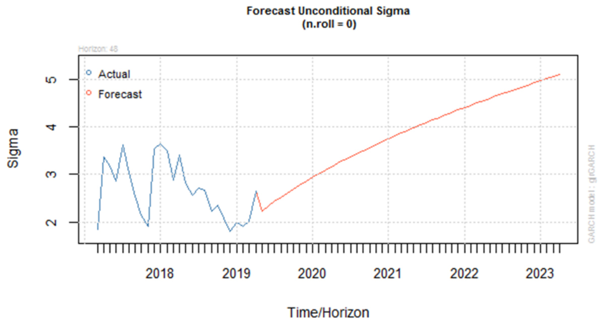
Figure 1: Forecast Plot with unconditional Sigma ( n.roll = 0 )
