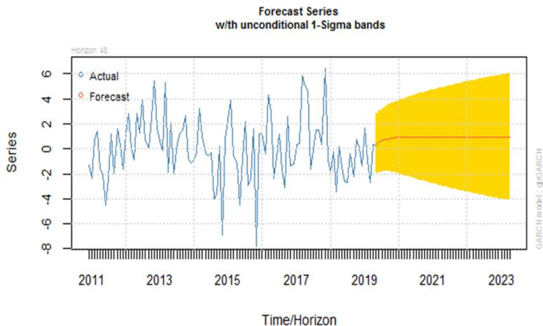
Figure 2: Forecast Plot with unconditional 1-Sigma bands
