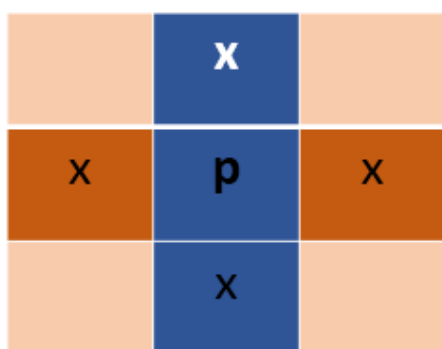
Fig. 2. 4-Connected Pixel
