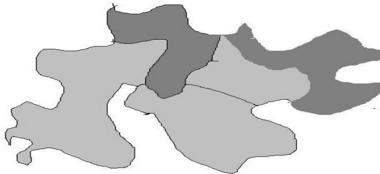
Fig.4. Input image
