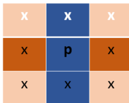
Fig. 3. 8-Connected Pixel
