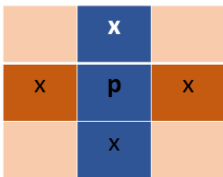
Fig. 2. 4-Connected Pixel
