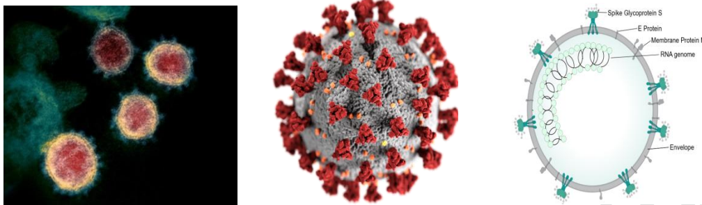
Figure 1: (a) Electron micrograph of SARS-CoV-2 virions with visible coronae (b). Illustration of a SARS-CoV-2 virion(c). Structure of a SARS-CoV-2 virion.(Source 1)
