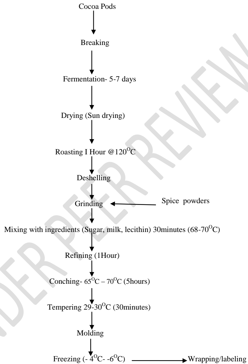
Fig 1. Flow Chart for Spicy chocolate Production [13]
