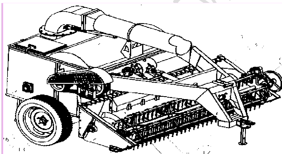
Figure 1: Schematic view of a Straw reaper combine
