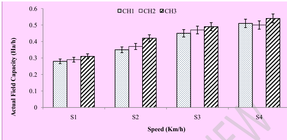
Figure: 4 Effect of cutting height and forward speed on actual field capacity
