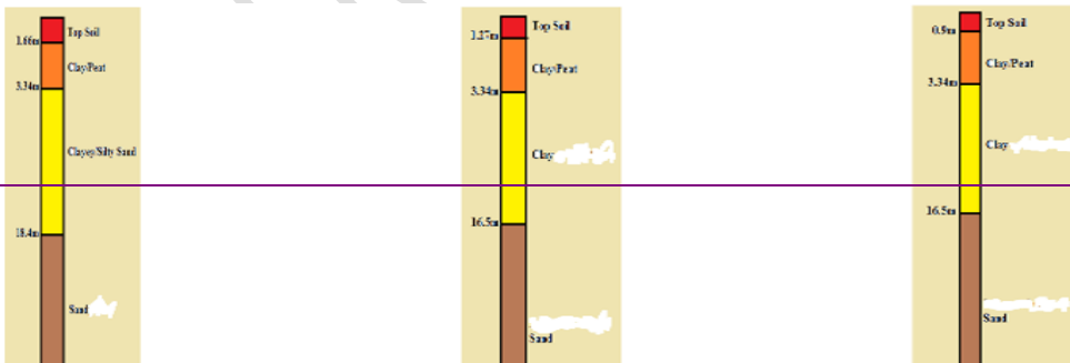
Fig. 24: Geo electric sections of VES 1-3 at location 3 (Agbara)
