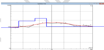
Fig. 16: VES 1 at Iyana Era
