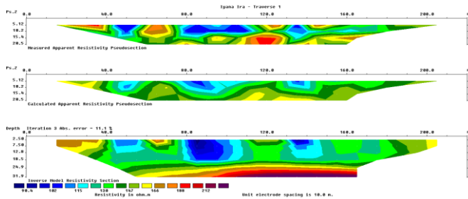
Fig. 7: Profile 1 at Iyana Era
