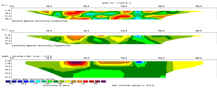
Fig. 9: Profile 3 at Iyana Era
