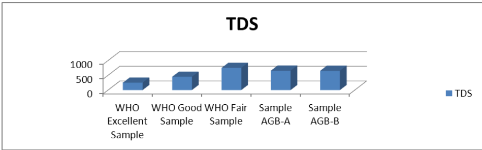
Fig. 24: Microsoft Excel chart showing the Total Dissolved solid compared to WHO at Location 3 (Agbara)
