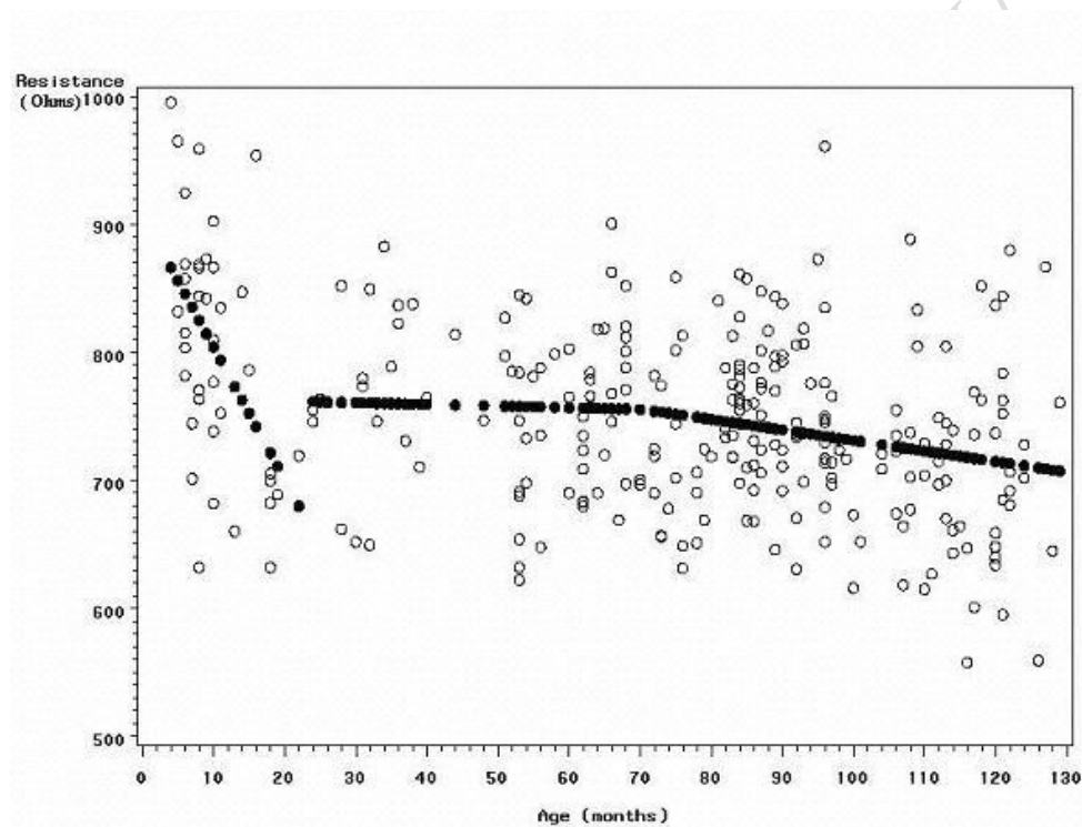
Figure 1– Relationship between measured (white) and predicted (black) Resistance values according to age. The regression line predicted for the three age groups studied were significantly different ( p = 0.0003 ).
