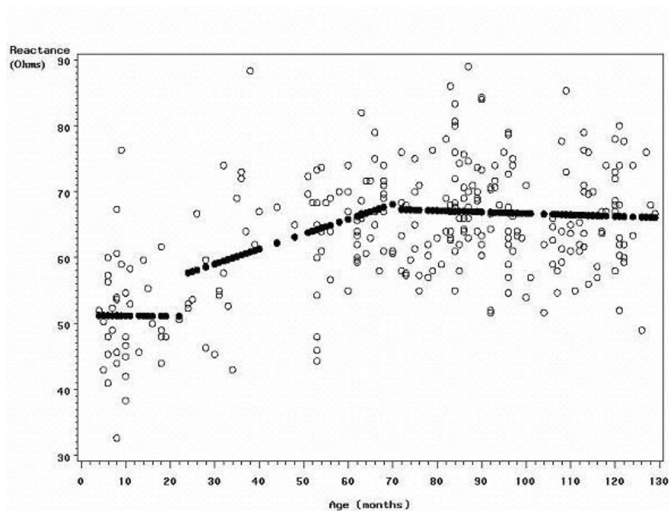
Figure 2 – Relationship between measured (white) and predicted (black) Reactance values according to age. The regression line predicted for the three age groups studied were significantly different ( p = 0.0065 ).
