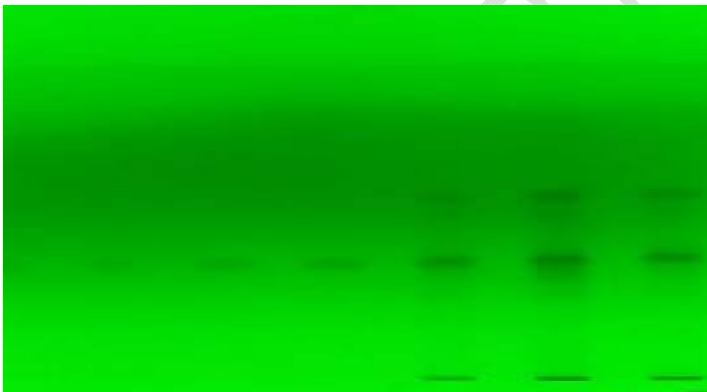
Figure -2: Picture showing spots of Trikatu Churna extract (track no.9) in comparison with piperine track no. 1-8.
