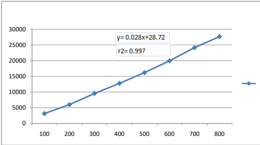
Figure-1 Calibration curve
