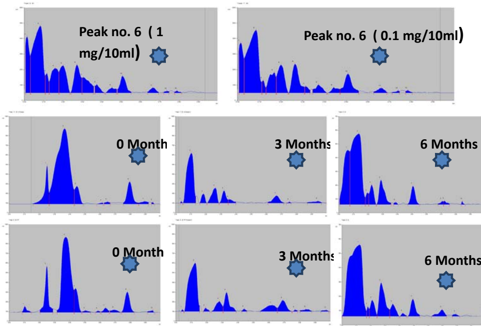
Figure-6: Freeze-Thaw Peak (1&2), Accelerated Stability Peak (3, 4 & 5) and Real-Time Peak (6,7 & 8)
