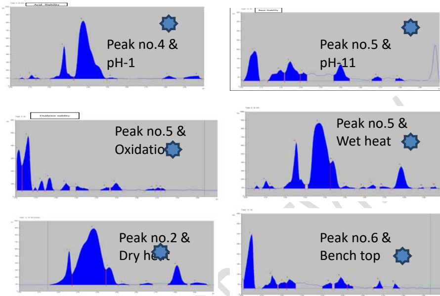
Figure – 5: Peaks of different stress degradation study (1-Acidic,2-Basic,3-Oxidation, 4-Wet heat, 5-Dry heat and 6-Bench Top)
