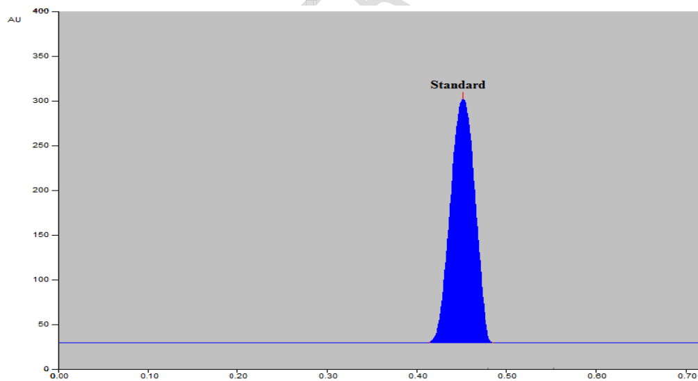
Figure 4: Standard piperine ( R_f = 0.46 )
