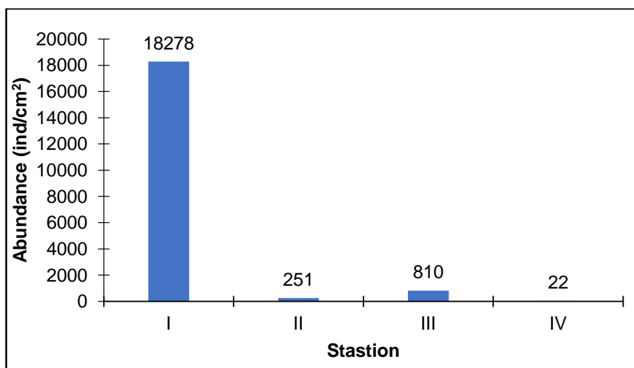
Fig 2. Abundance of Citarik River Periphyte during Research
