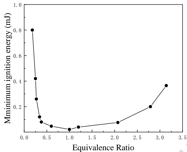
Fig.2. The relationship between the equivalence ratio and the minimum ignition energy.
