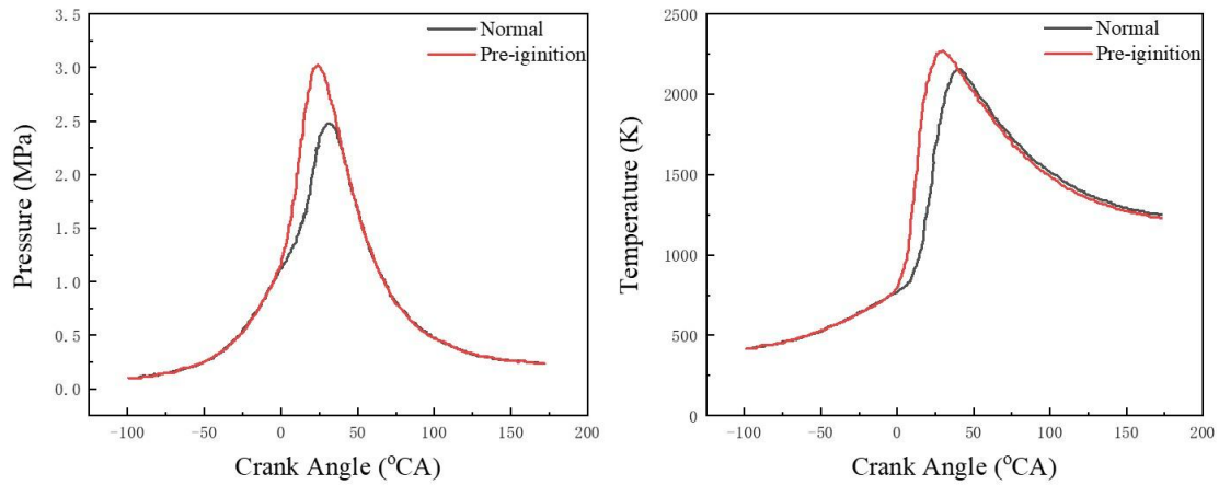
Fig.1. Changes in cylinder temperature and pressure for normal combustion and pre-ignition
