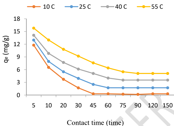
Fig 3. Effect of contact time and temperature on the removal of SMT by TTRH (concentration: 50 mg/L; dose: 2.5 g/L; shaking speed: 180 rpm; pH: 7)
