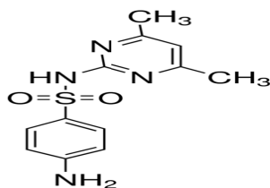
Fig.1. Molecular structure of Sulfamethazine (SMT)
