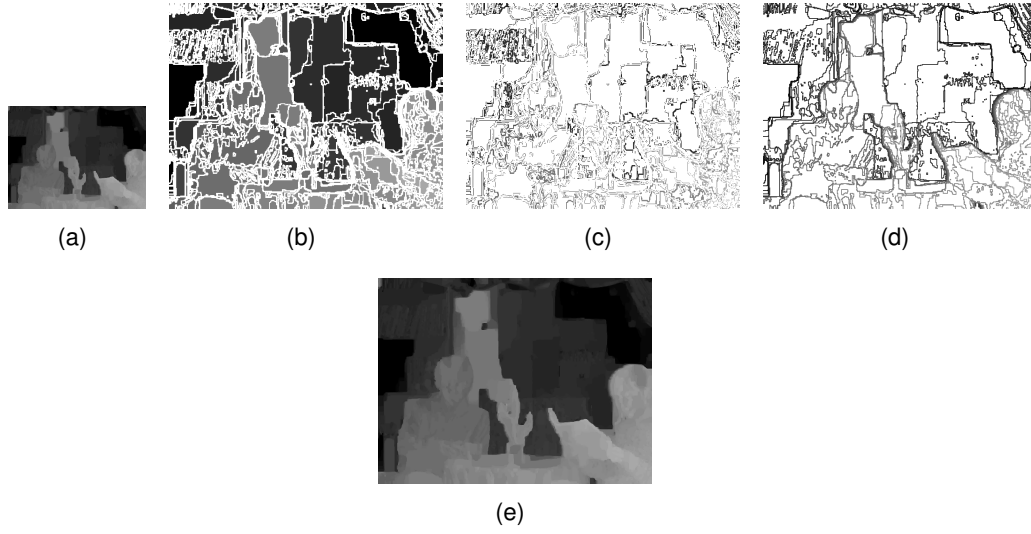
Figure 2: The sketch of our region-based depth map upsampling method. (a) The given low-resolution depth map. (b) The reconstructed homogeneous depth pixels, which occupy 73% of all reconstructed pixels, by our DC copying approach. (c) The reconstructed semi-homogeneous depth pixels, which occupy 12% of all reconstructed pixels, by our MV approach. (d) The reconstructed non-homogeneous depth pixels, which occupy 15% of all reconstructed pixels, by using BIC. (e) The constructed high-resolution depth map by our “DC+MV+BIC” method.
