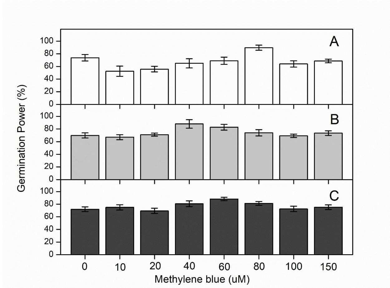
Figure 1: Germination power of cowpea (A), millet (B) and sorghum (C) seeds after 48 h, having previously primed for 6 h in different concentrations of MB.
