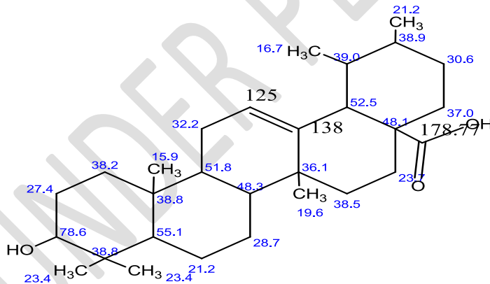
3-Hydroxyurs-12-en-28-oic acid.
